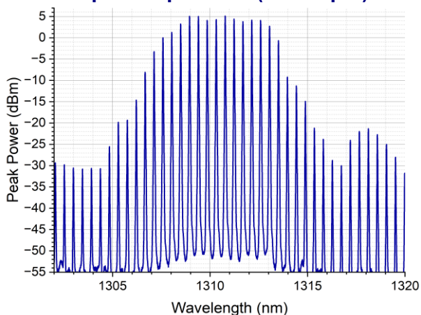
Optical Spectrum (res. 10pm)
