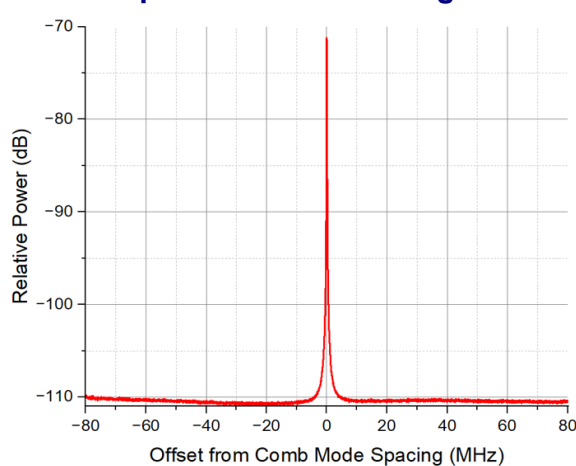
RF spectrum of all beating modes
