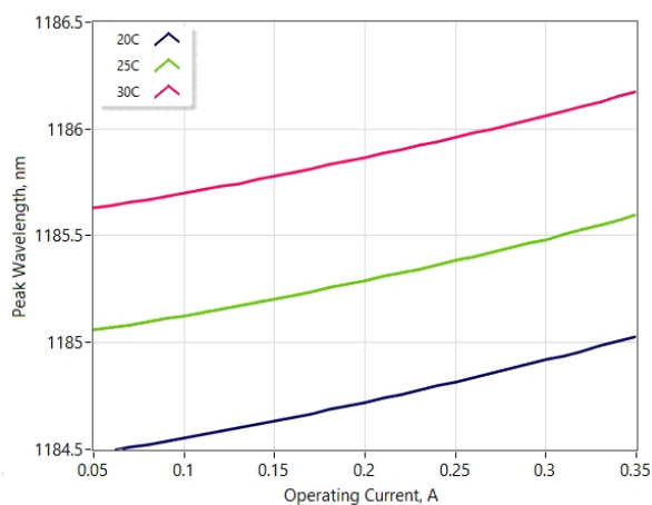
Peak Wavelength Tuning by Current
