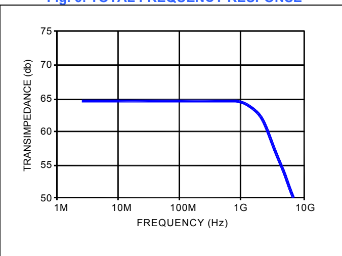
Fig. 6: TOTAL FREQUENCY RESPONSE
