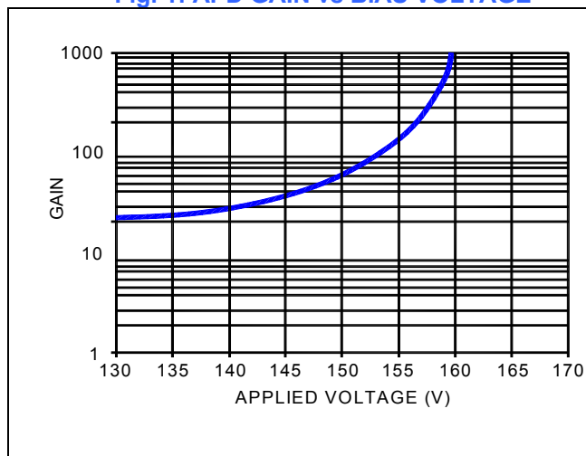
Fig. 1: APD GAIN vs BIAS VOLTAGE
