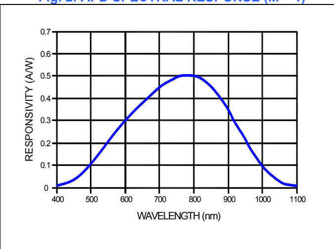
Fig. 2: APD SPECTRAL RESPONSE (M = 1)
