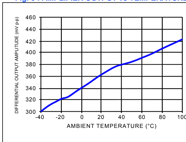
Fig. 3 : AMPLIFIER OUTPUT vs TEMPERATURE
