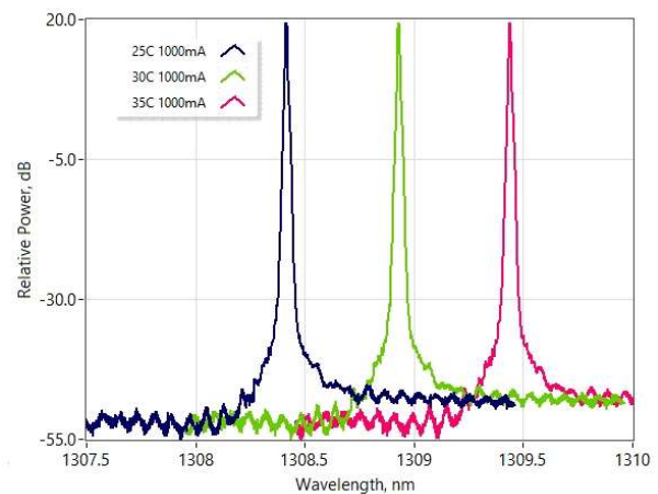
Optical Spectra vs Temperature (res. 5pm)
