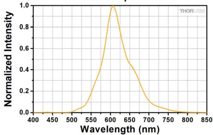
M595D3 Spectrum
