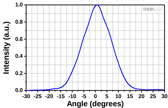
LEDW7E Far Field Distribution
