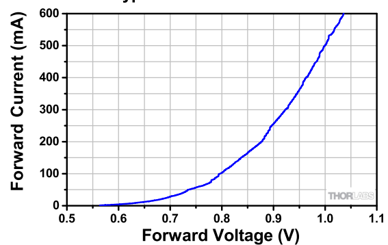
Typical Forward Current
