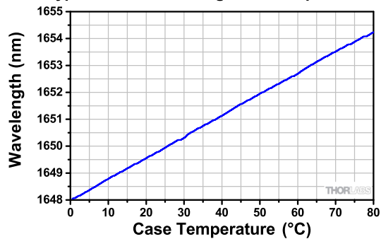
Typical Peak Wavelength vs. Temperature
