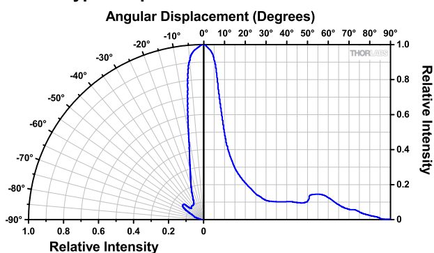
Typical Spatial Radiation Distribution
