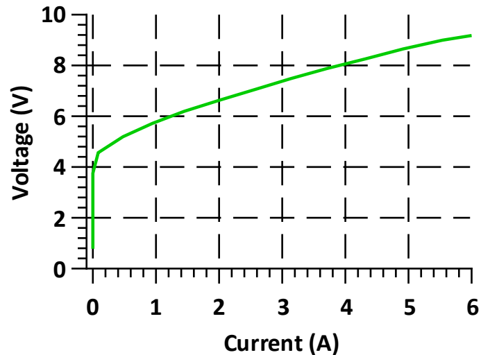
Figure 3: Typical V_F vs. i_F
