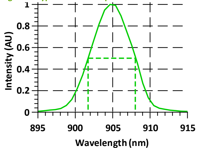
Figure 5: Typical Emission Spectrum
