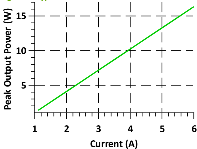
Figure 2: Typical P vs. i_F
