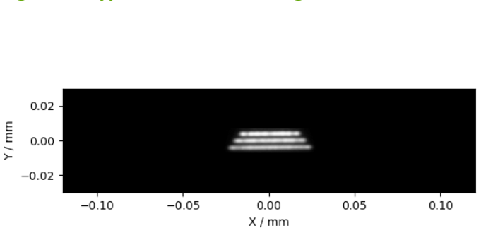
Figure 9: Typical Near Field Image
