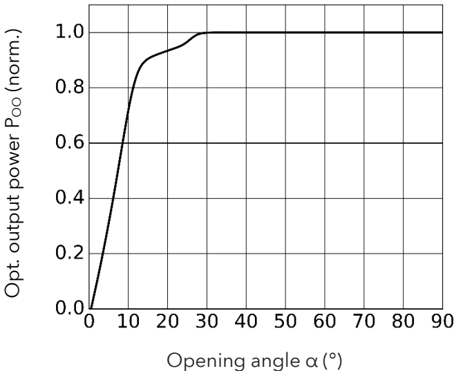
Normalized optical output power 7 P_{OO} (integral from 0^{\circ} to \alpha ) versus opening angle \alpha
