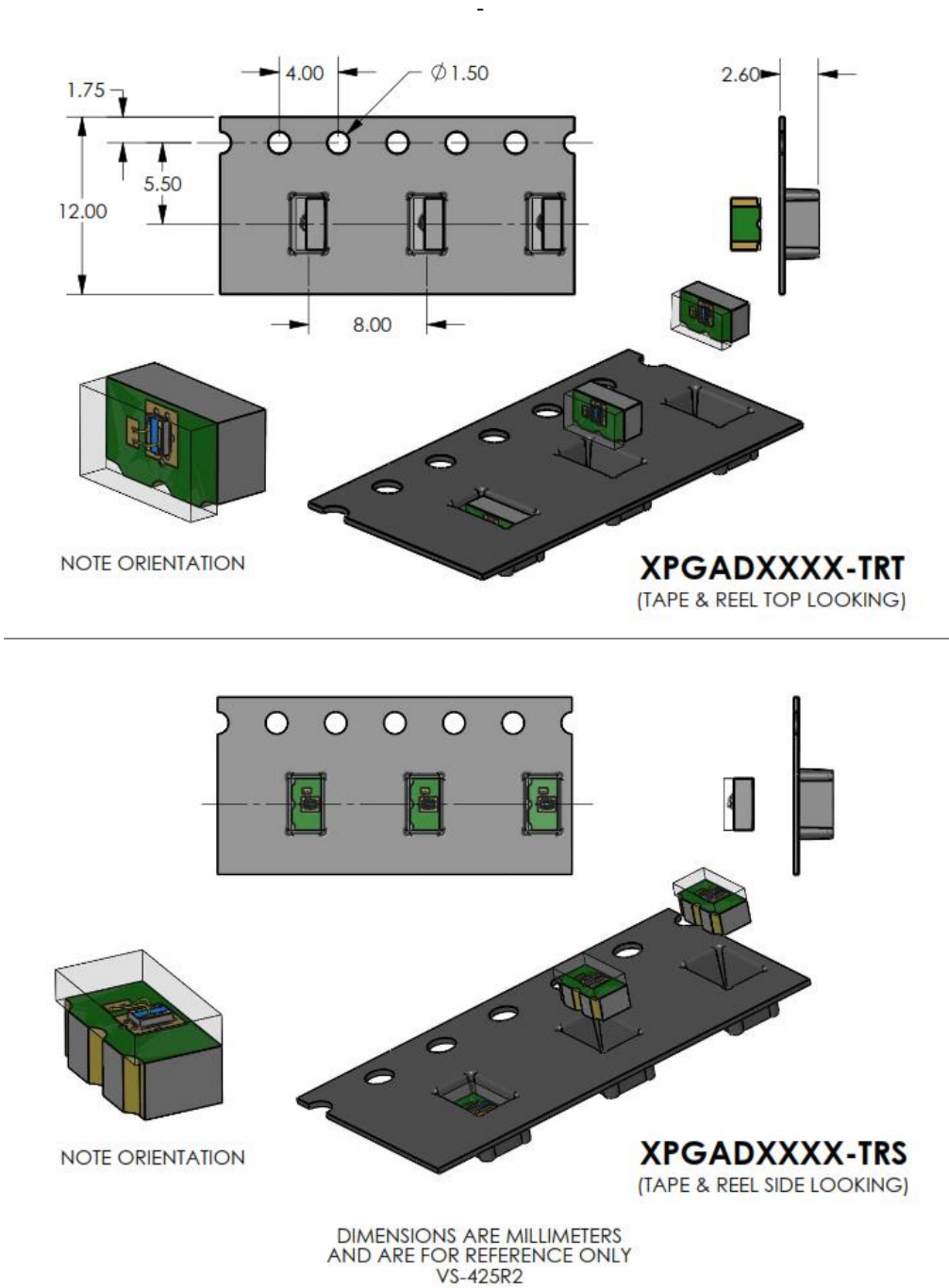
Figure 8: Tape and Reel Packaging Dimensions
