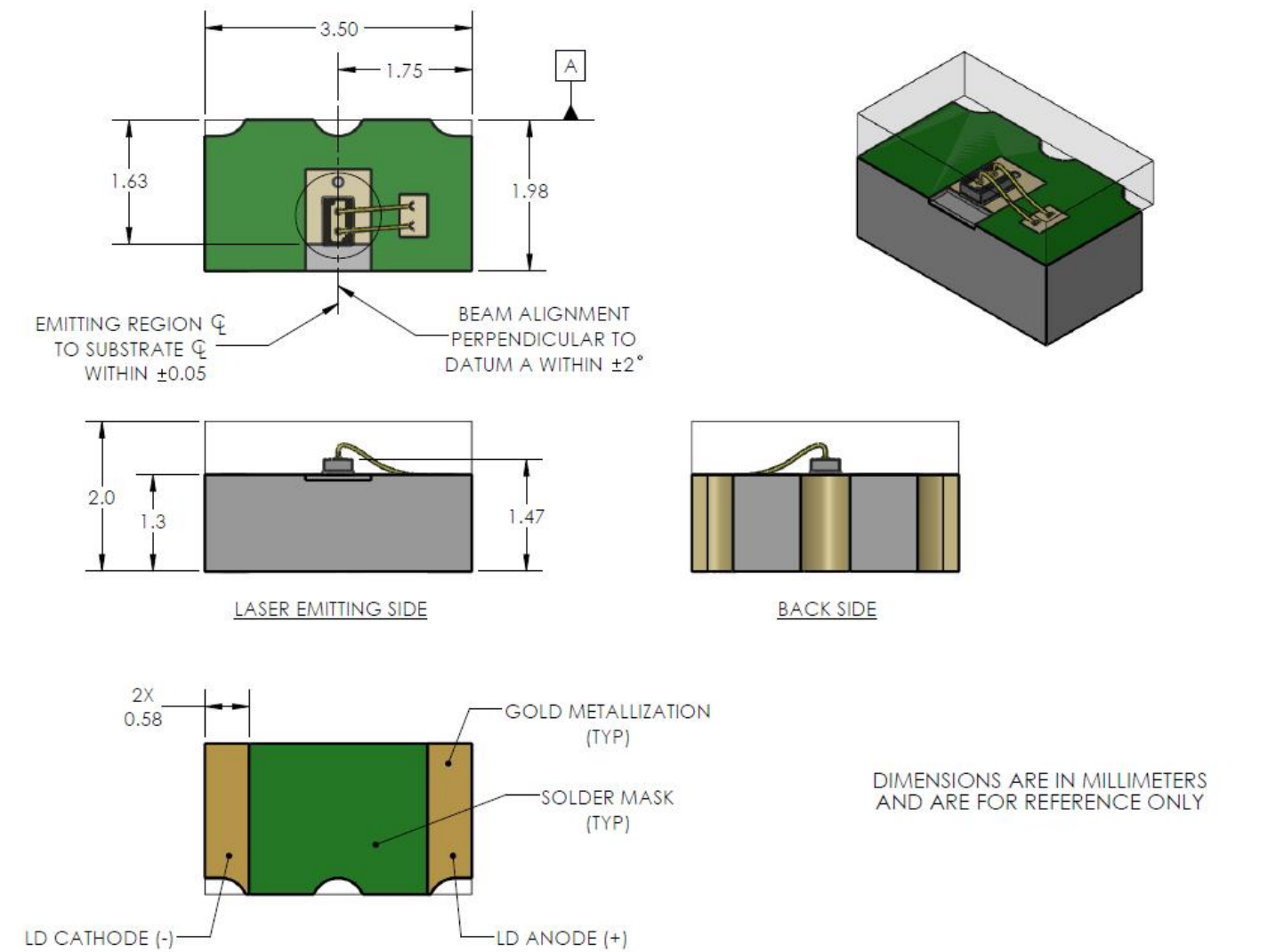
Figure 1: Laser Package Dimension TPG3AD1S09
