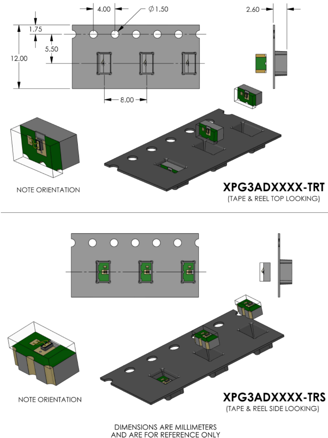
Figure 8: Tape and Reel Packaging Dimensions
