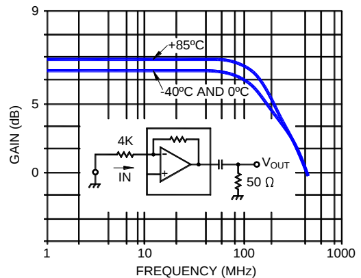
Fig. 6: AMPLIFIER GAIN vs. FREQUENCY
