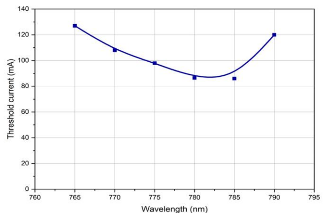
Threshold current
