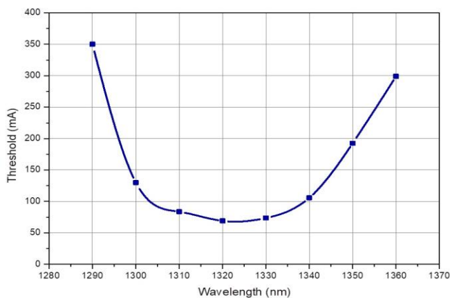
Threshold current
