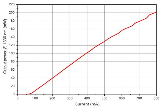
Output power @ 1330nm
