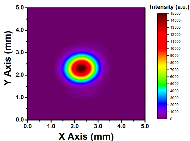
QD7416HH Sample Beam Profile
