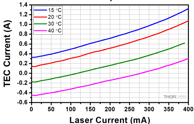
QD7416HH Sample TEC Current
