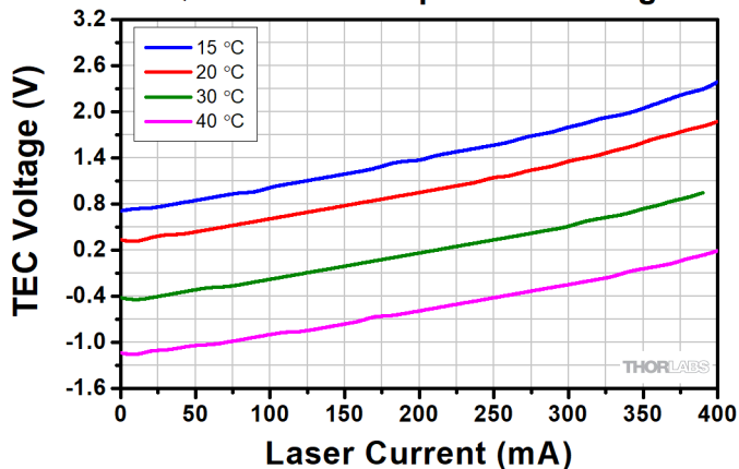
QD7416HH Sample TEC Voltage
