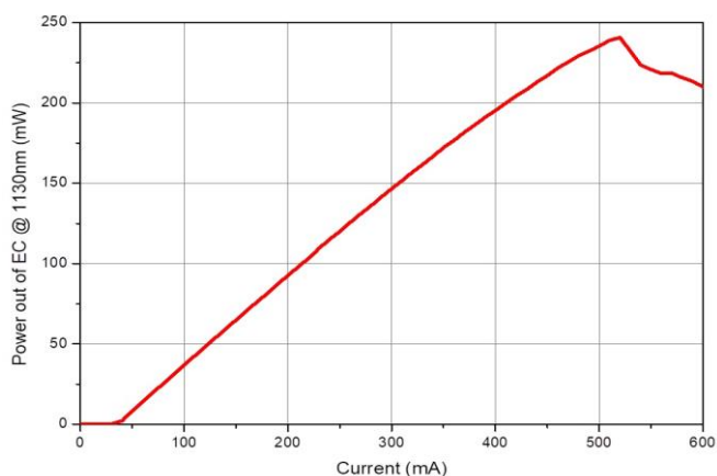
Output power @ 1130nm
