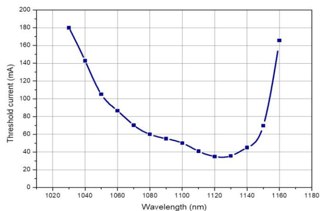
Threshold current
