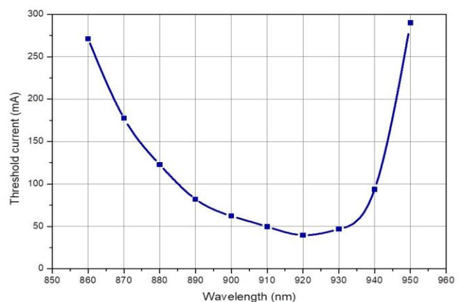
Threshold current
