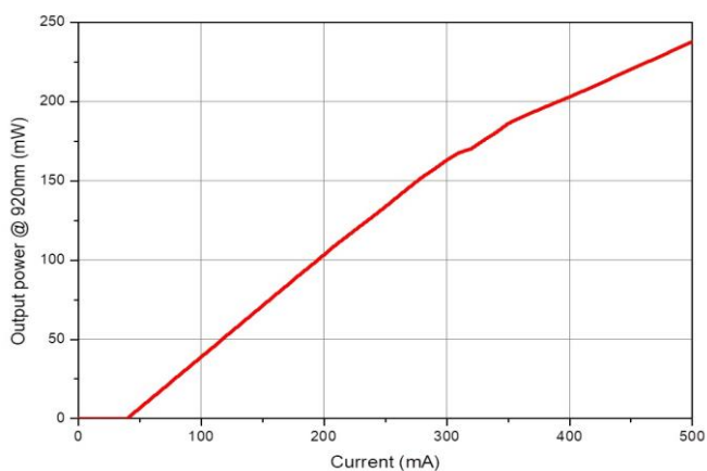
Output power @ 920nm
