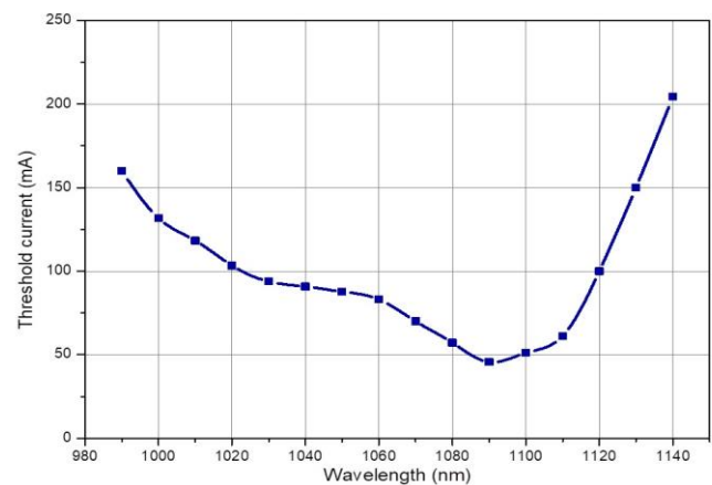
Threshold current
