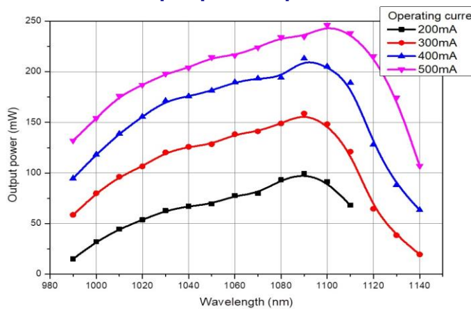
Output power spectra
