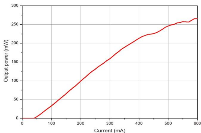
Output power @ 1090nm
