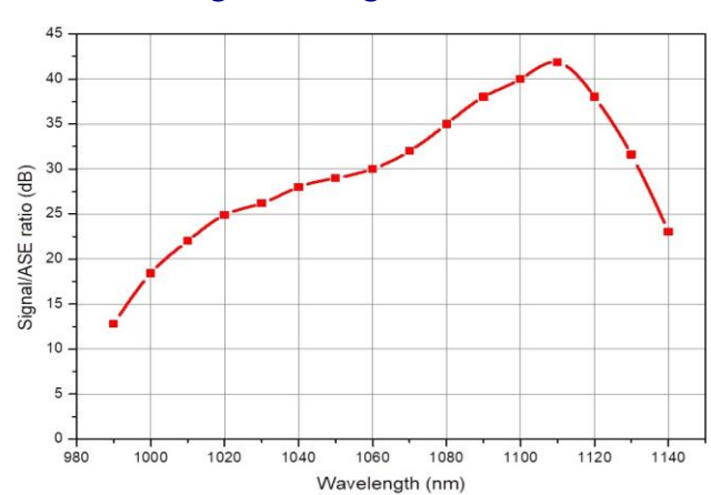
Integrated Signal/ASE ratio
