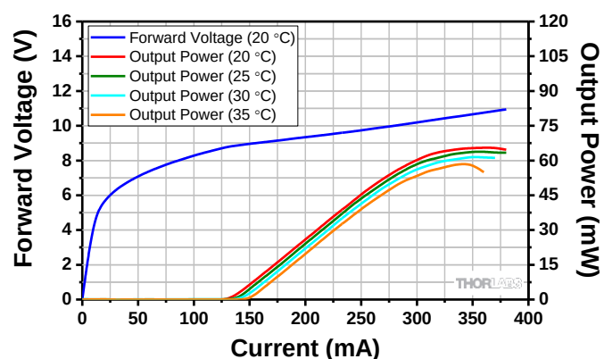
QD6134HH Sample L-I-V Characteristics
