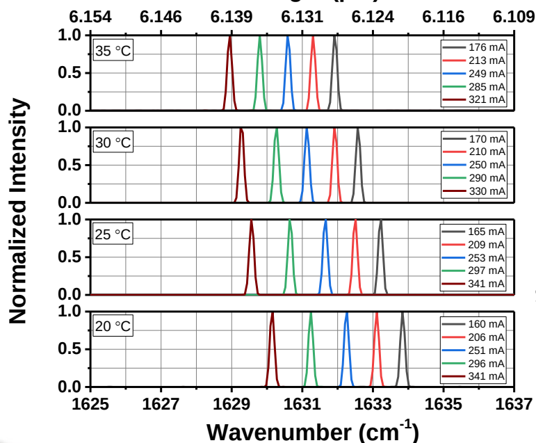
QD6134HH CW Spectral Characteristics
