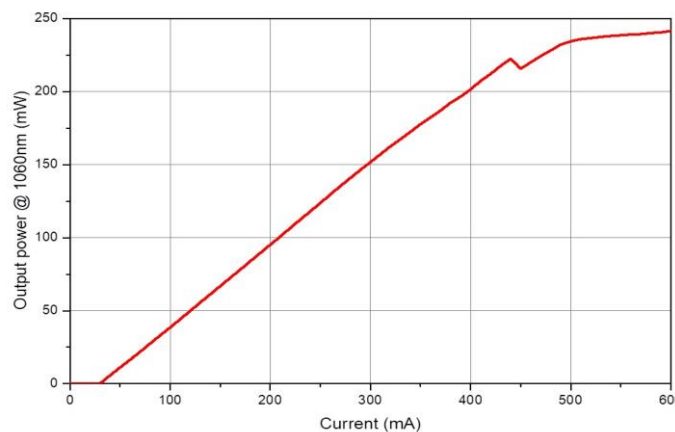
Output power @ 1060nm
