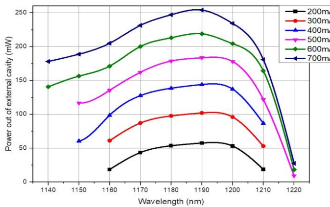
Output power spectra
