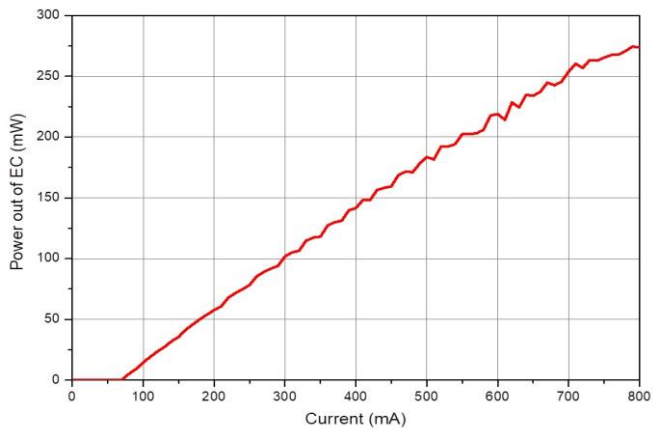
Output power @ 1190nm
