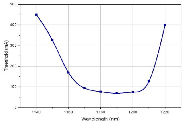
Threshold current
