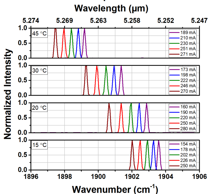
QD5263HH CW Spectral Characteristics
