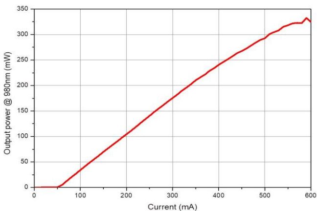
Output power @ 980nm
