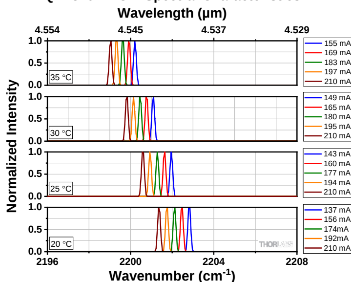
QD4540HH CW Spectral Characteristics
