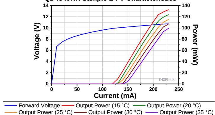
QD4540HH Sample L-I-V Characteristics
