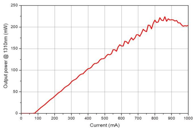
Output power @ 1310nm
