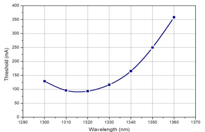
Threshold current
