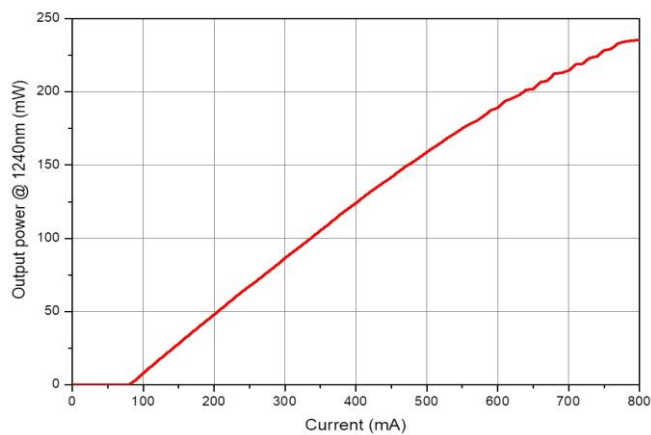
Output power @ 1240nm
