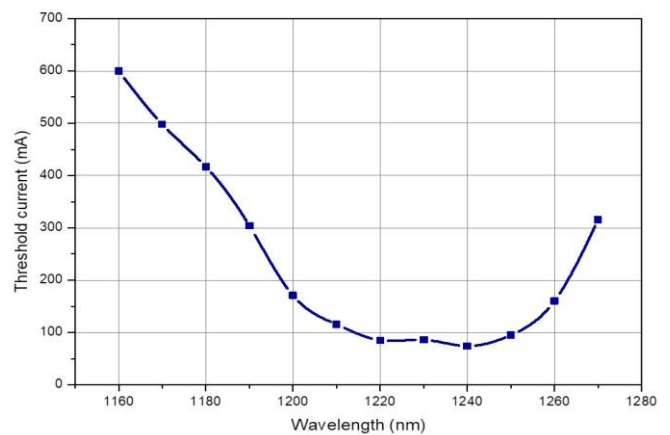
Threshold current
