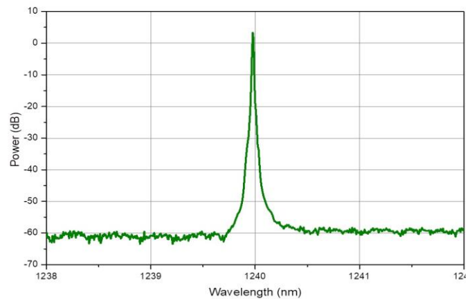
Optical spectrum (res. 10 pm)
