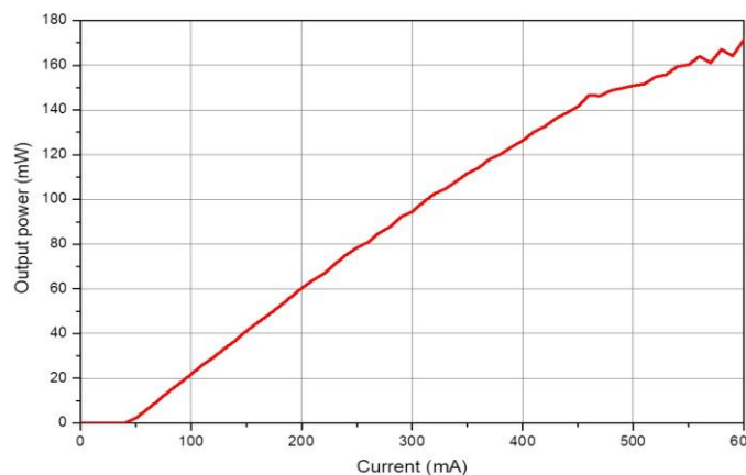
Output power @ 1260nm
