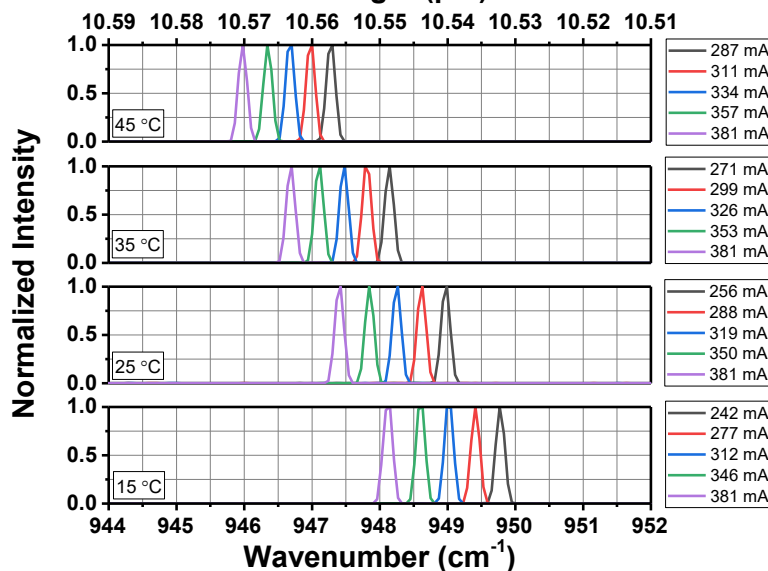
QD10549HH CW Spectral Characteristics
