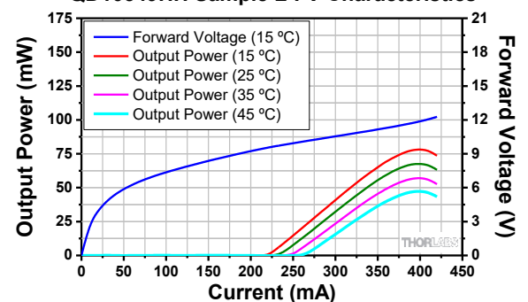
QD10549HH Sample L-I-V Characteristics
