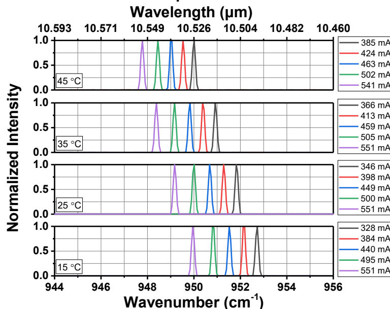
QD10530HH CW Spectral Characteristics
