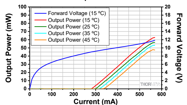
QD10530HH Sample L-I-V Characteristics
