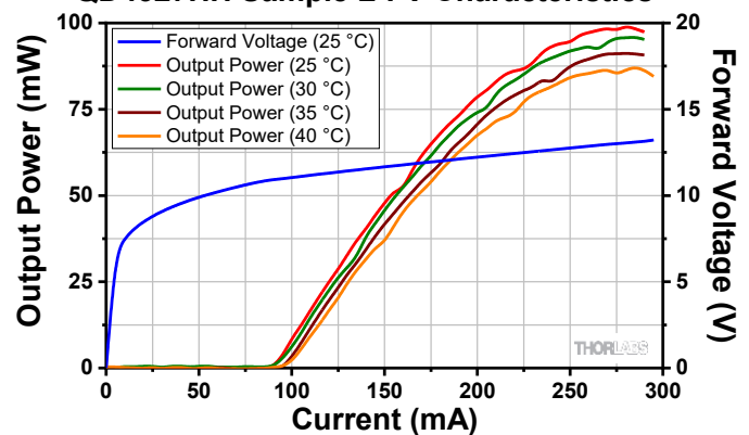
QD4327HH Sample L-I-V Characteristics
