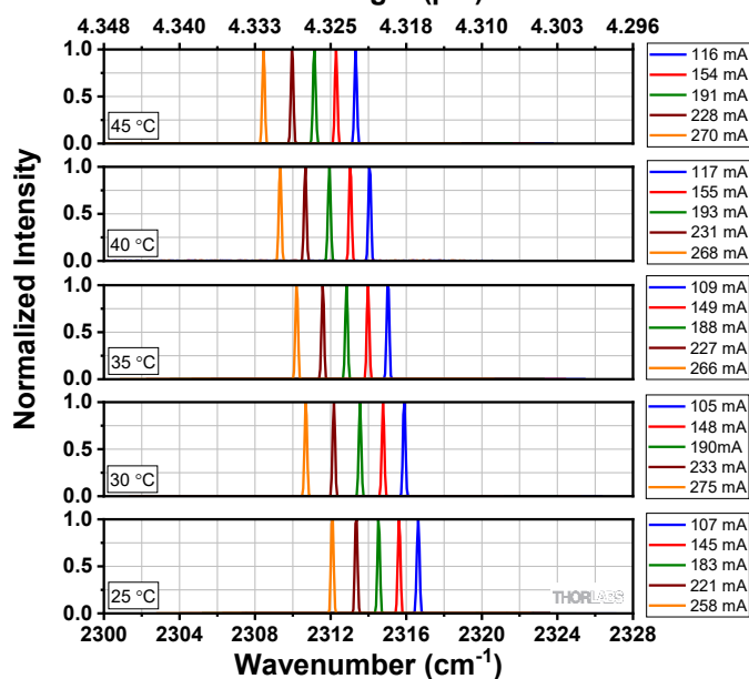
QD4327HH CW Spectral Characteristics Wavelength ( \mu\text{m} )
