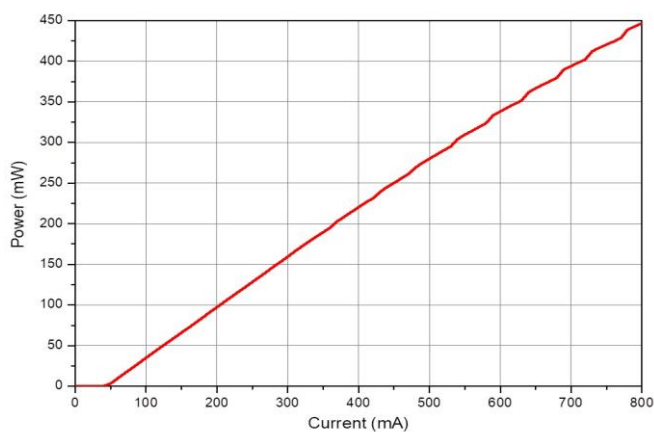
Output power @ 1120nm
