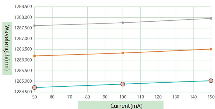
Tuning Characteristics
