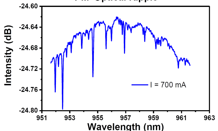
PM Optical Ripple
