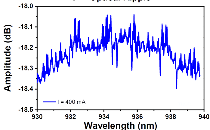
SM Optical Ripple
