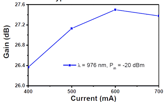
Typical Gain vs. Current
