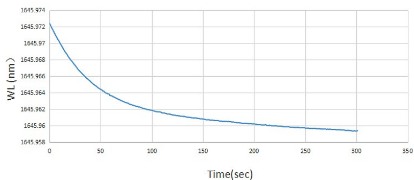
5mins Wavelength stability Test
