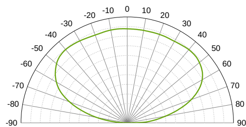
View Angle Abstrahlung
