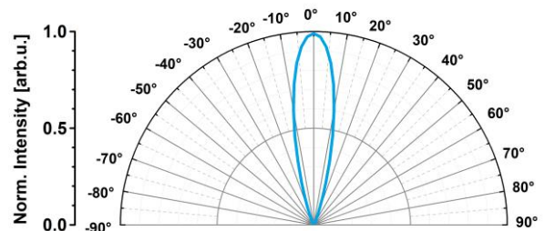
Radiation Pattern
