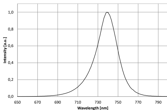
Relative Spectral Emission Spektrum
