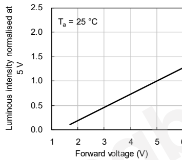
Luminous Intensity vs. Forward Voltage
