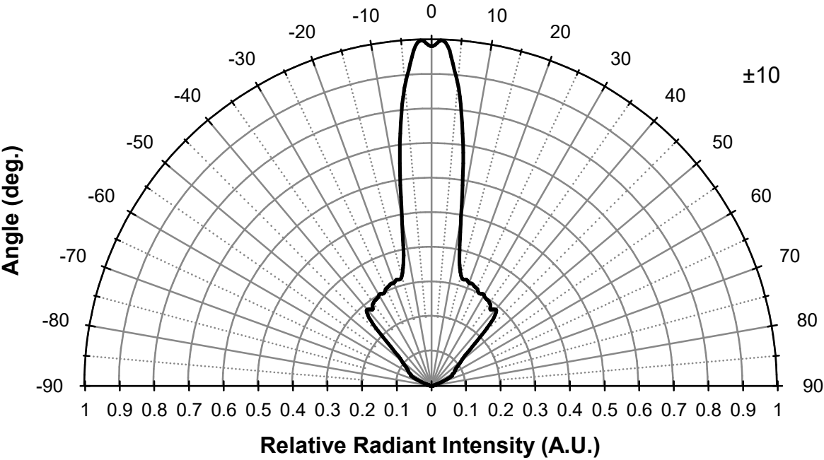
Radiation Characteristics
