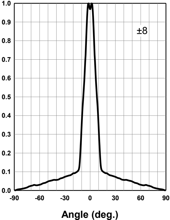
Radiation Characteristics
