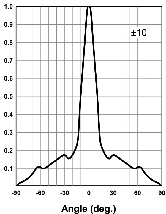
Radiation Characteristics
