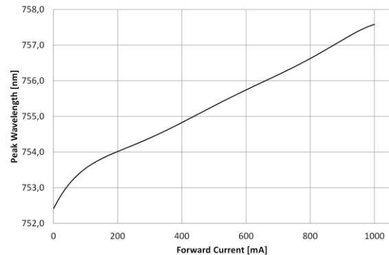
Wavelength Shift vs. Forward Current
