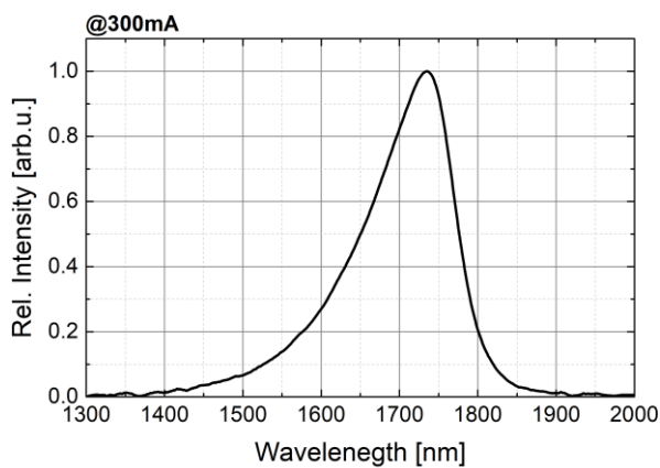
Optical Spectrum
