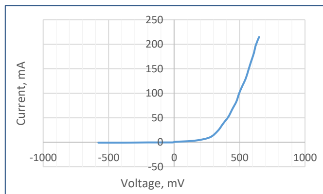
Typical current-voltage characteristic ( \text{qCW}^2 )
