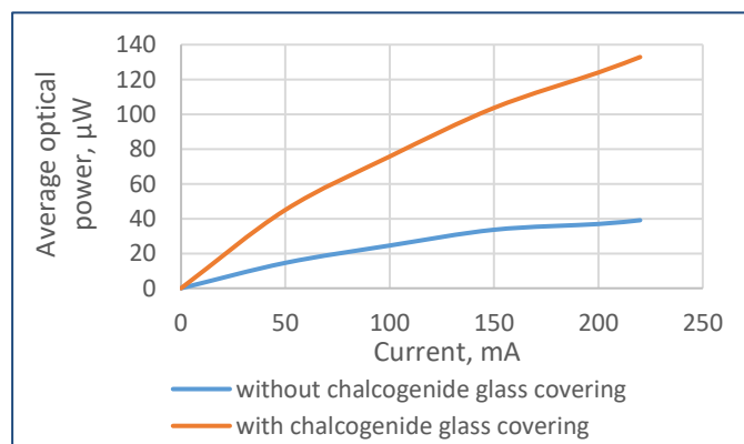
Typical optical power - current characteristic ( \text{qCW}^2 )
