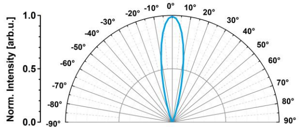
Radiation Pattern
