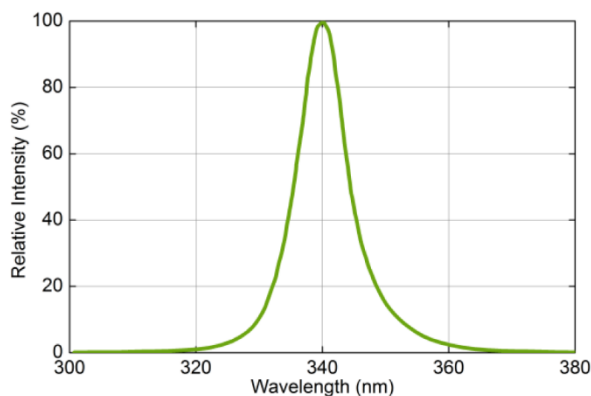
Optical Spectrum
