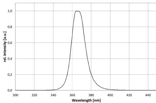
Spectrum @ 20mA Spektrum @ 20mA
