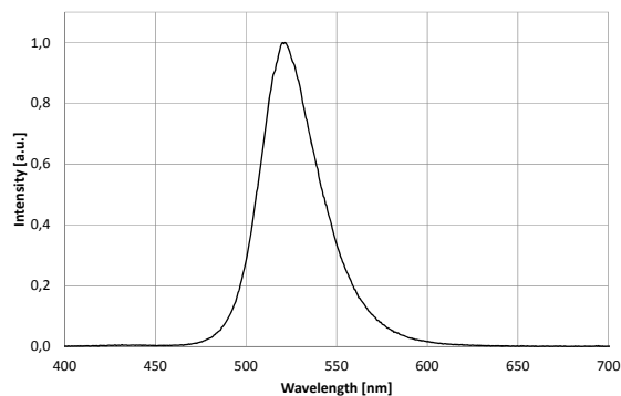
Spectrum @ 25°C Spektrum
