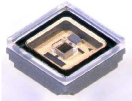
Ceramic SMD Ultraviolet LED with Flat Top
